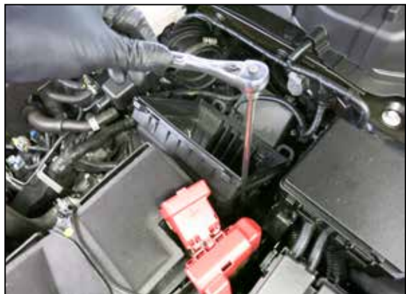
7. Loosen the bolt that secures the lower air filter housing to the bracket and then remove the lower housing from the vehicle.
