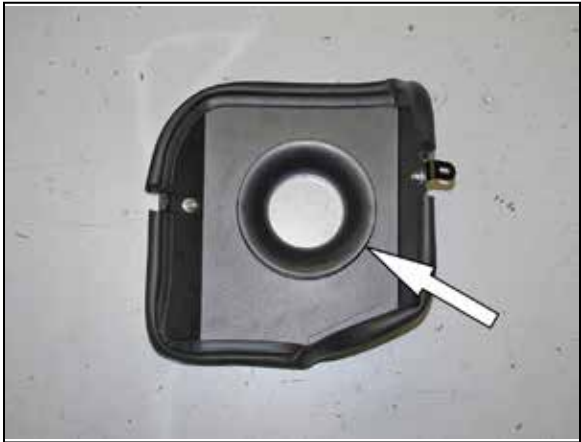
11. Install the filter adapter into the heat shield and secure with the provided hardware.
