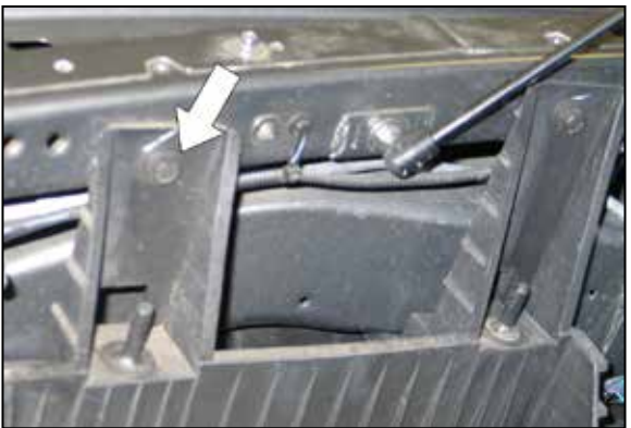
17. Remove the front air box mounting bracket bolt shown. NOTE: This bolt will be used in a later step.
