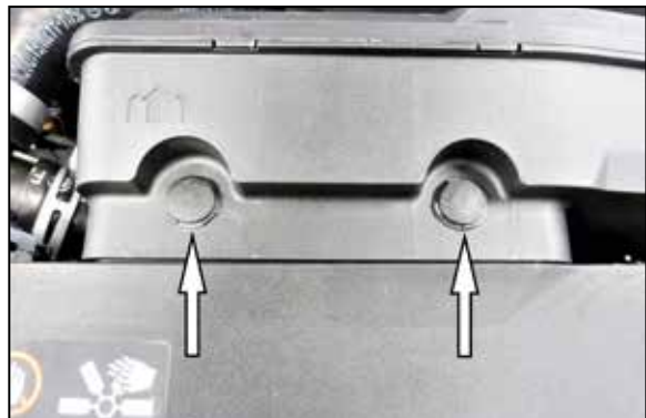
5. Pop up the centers of the fresh air duct retaining pins and then remove the pins from the vehicle.
