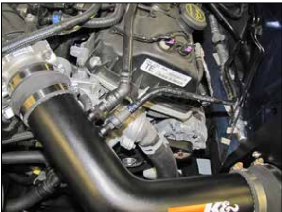
15. Connect the EVAP and crank case vent lines to the quick disconnect fittings as shown.
