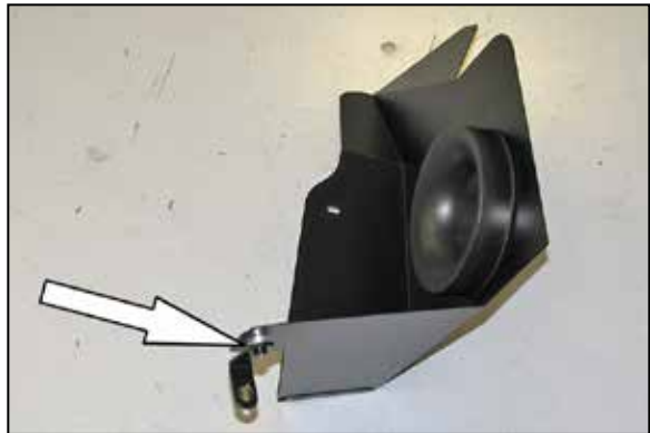
7. Install the provided heat shield bracket (064326) onto the heat shield and secure with the provided hardware. NOTE: be sure to place the provided spacer between the bracket and heat shield.
