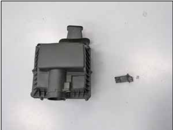
16. Remove the two screws securing the mass air sensor and then remove the mass air sensor from the factory air filter housing.
