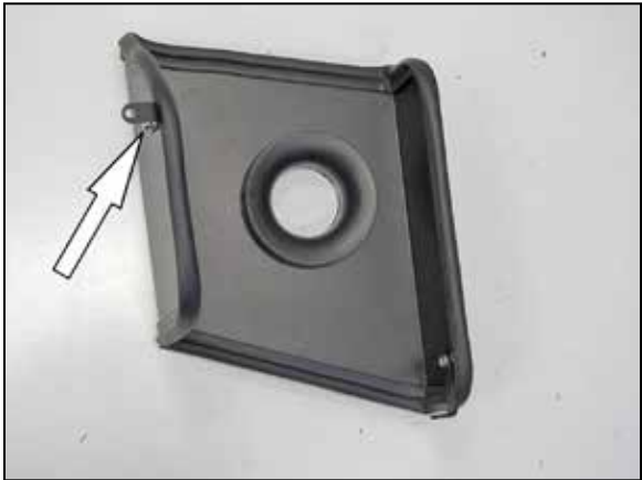
13. Install the heat shield mounting bracket (07805A) onto the heat shield using the provided hardware and spacer. NOTE: The spacer is to be placed between the heat shield and bracket.
