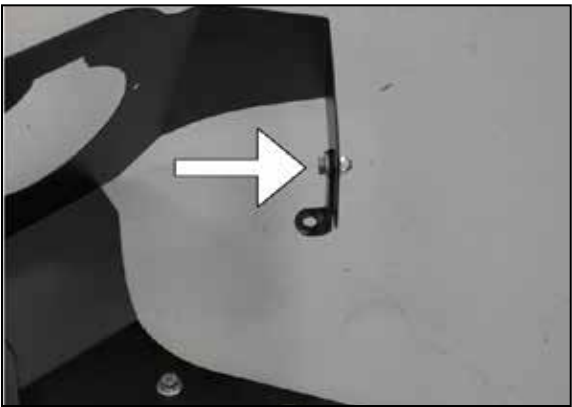
9. Install the heat shield mounting bracket (07158A) onto the heat shield using the provided hardware.
