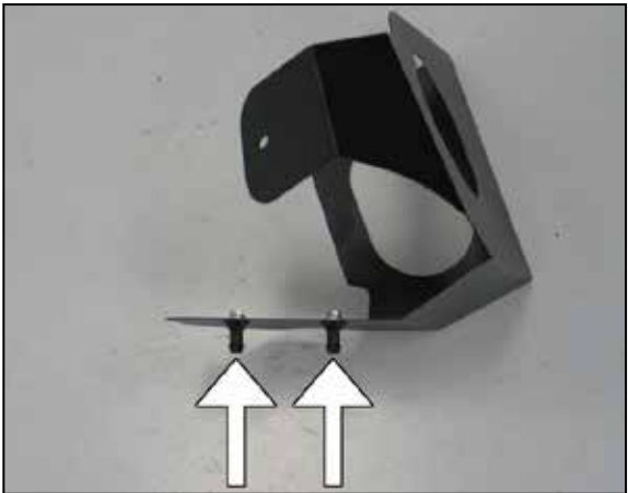
8. Install the heat shield mounting posts to the heat shield using the provided hardware as shown.
